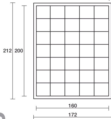
Piano letto e massimo ingombro Bed surface and max space occupied
